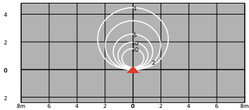
Isolux distribution on ground - fixture height 0.5m
