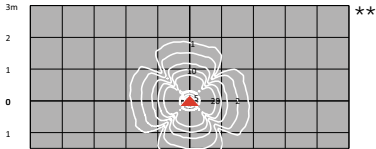
isolux distribution on ground - fixture height 0.2m
